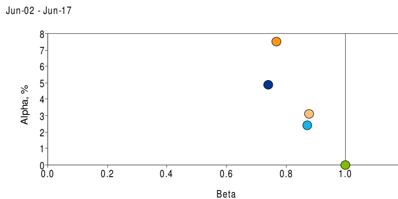
Alpha vs. Beta
